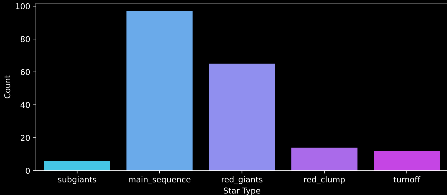
APOGEE DR17 Field: [K2_C18_214+26_btx] Count plot of Star Type
