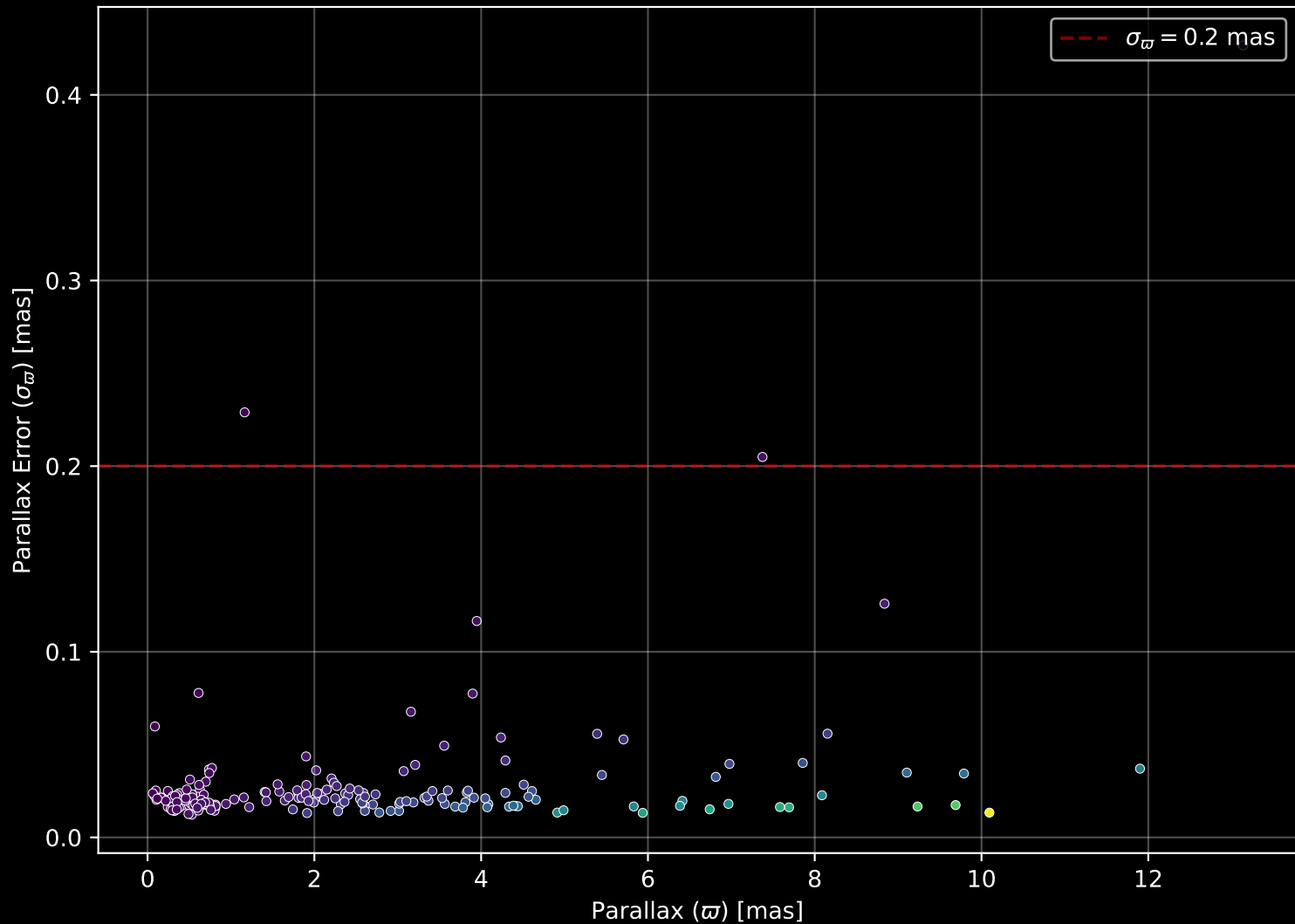
APOGEE DR17 Field: [K2_C18_214+26_btx] Parallax Quality (n= 194)
