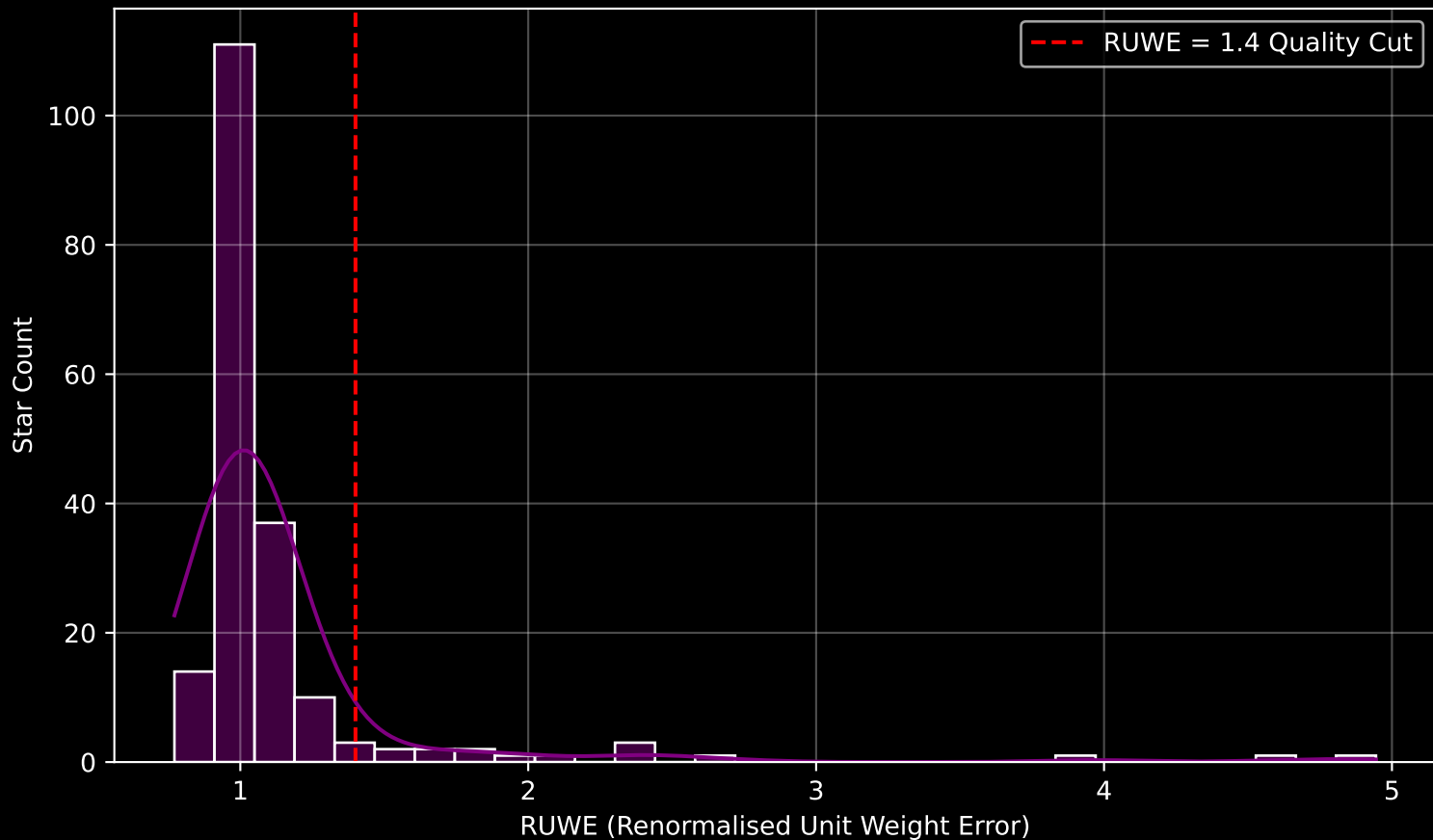
GAPOGEE DR17 Field [K2_C18_214+26_btx] RUWE Distribution (n= 190)
