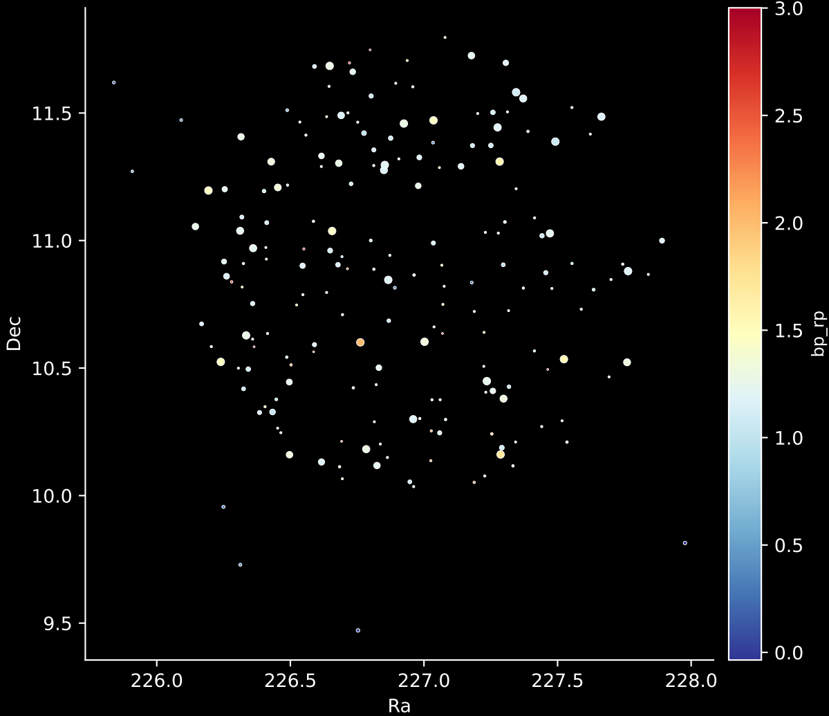
APOGEE DR17 Field: [K2_C18_214+26_btx] Stars: 194
