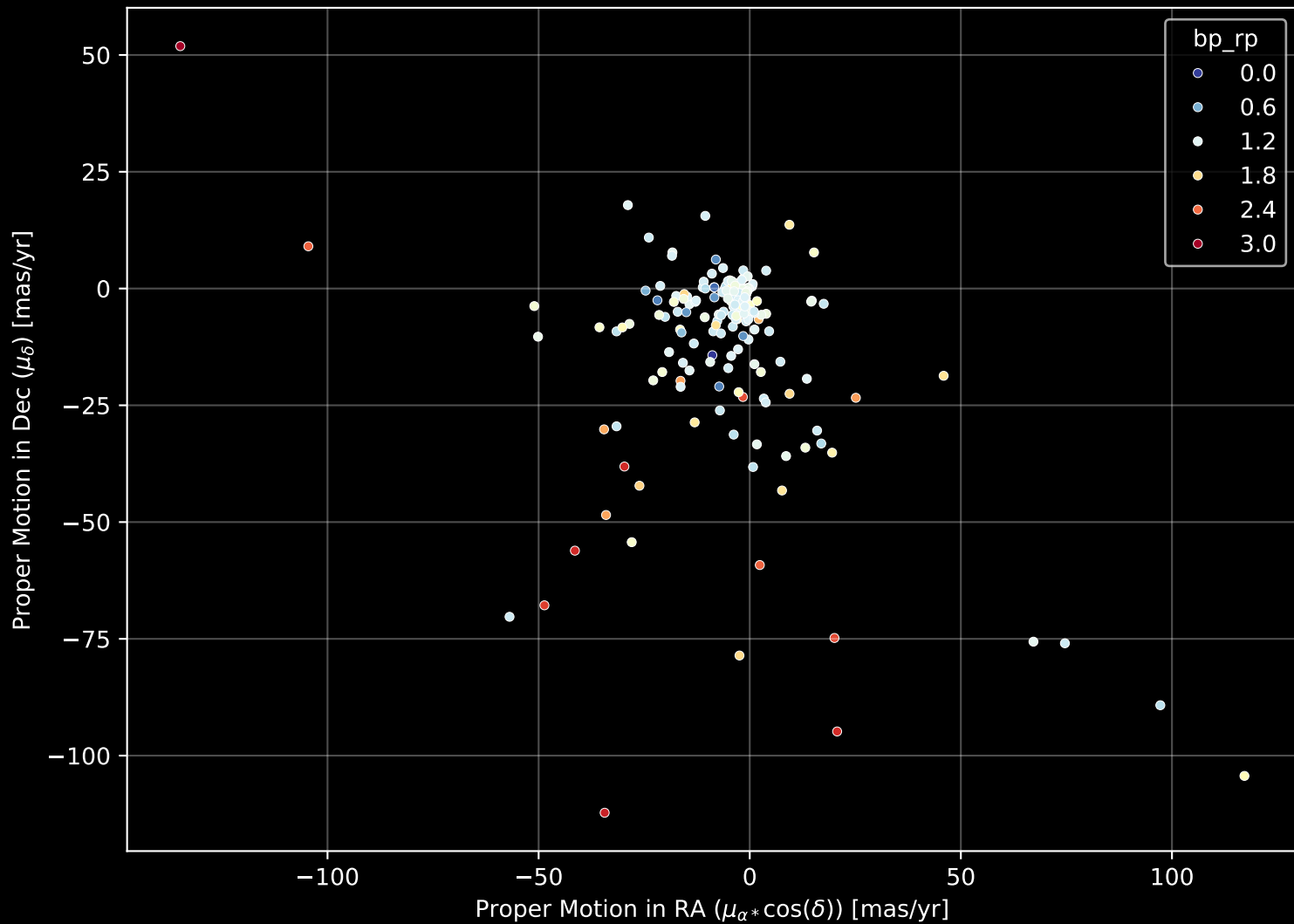
APOGEE DR17 Field: [K2_C18_214+26_btx] Proper Motion Diagram (n= 194)
