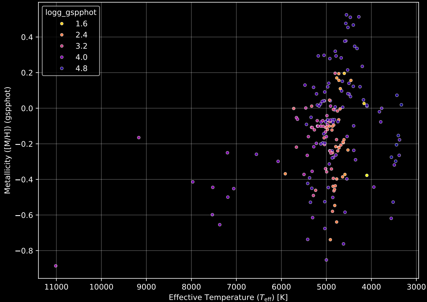
APOGEE DR17 Field: [K2_C18_214+26_btx] Stellar Population Parameters (n= 194)
