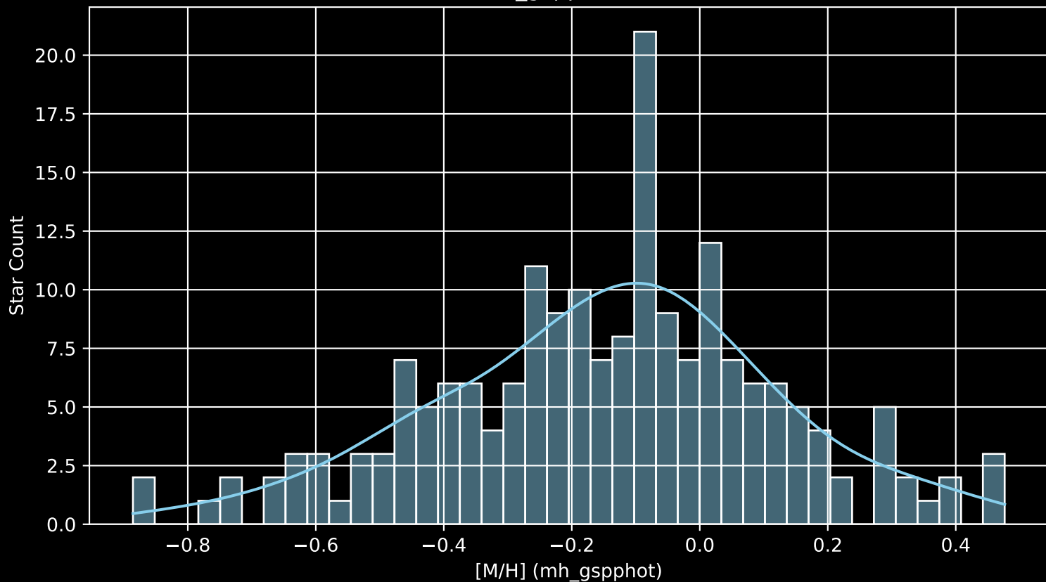
APOGEE DR17 Field: [K2_C18_214+26_btx [M/H] (mh_gspphot) (n= 191)
